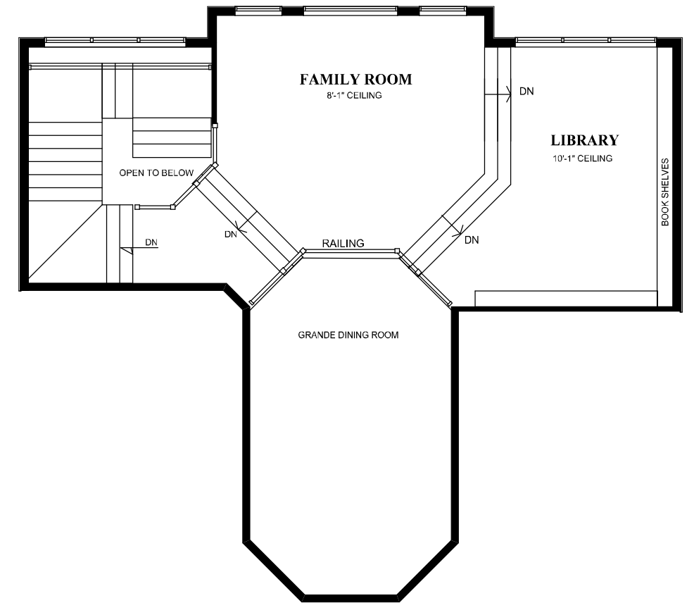
LOFT PLAN 550 SQ. FT.
